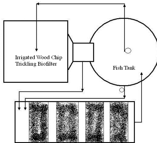
Submerged Filter Bioreactor
